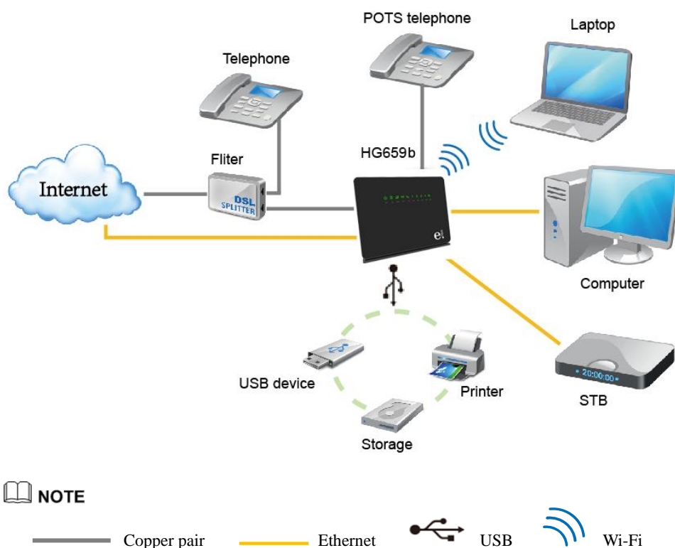
Figure 1-4 Networking diagram of the eir F2000 eir Fibre Modem
